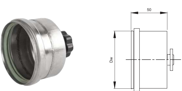
STOPPER
