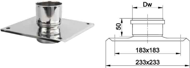
CHIMNEY PLATE
